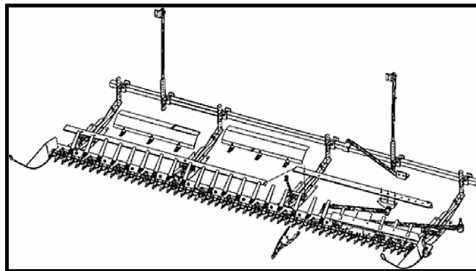
J.E. Love Floating Cutterbar
